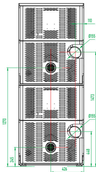
REAR VIEW
