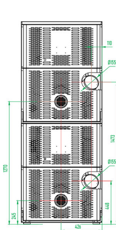
REAR VIEW
