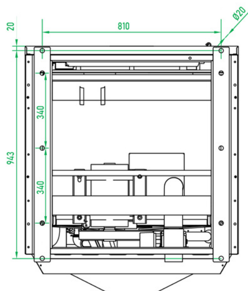
BOTTOM VIEW
