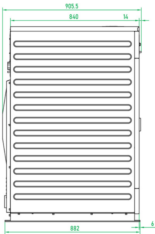
SIDE VIEW
