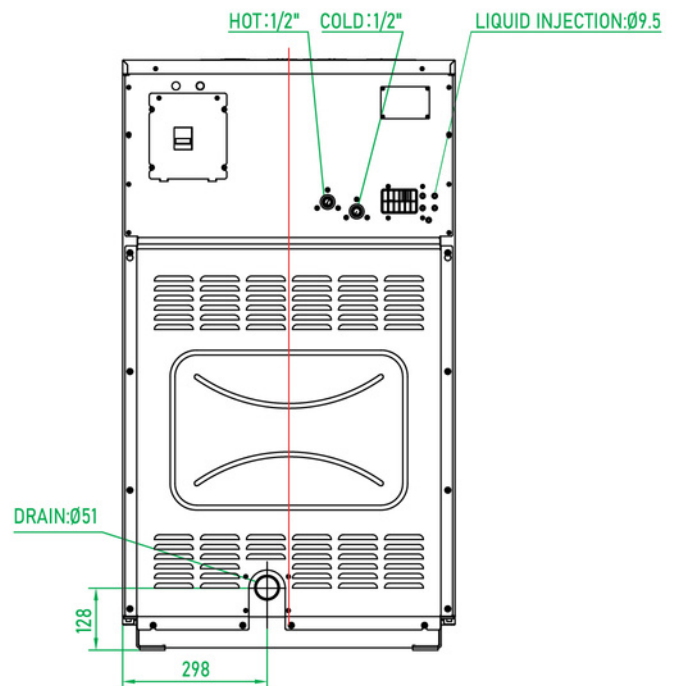
REAR VIEW
